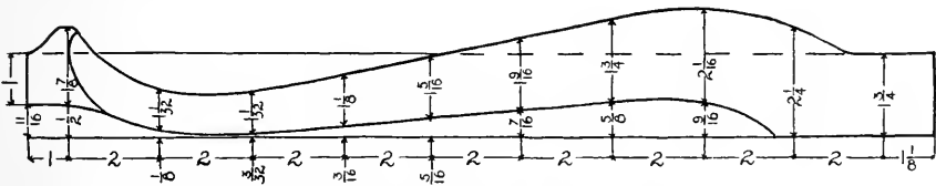
FIG. 390. MODIFIED LOUIS XV STYLE OF LEG.
